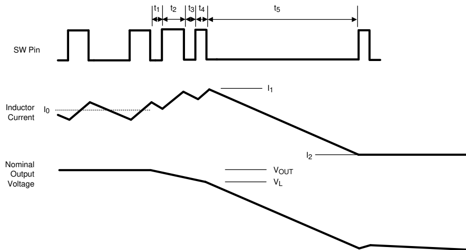
Figure 21. Fault Condition Timing
